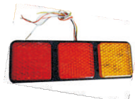
TL0120 LED tail light Stop, rear position, rear direction indicator lamp 100% waterproof Size: 274×94×28mm
