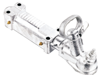
TC2014 Australia trailer coupler Ball size:50mm
