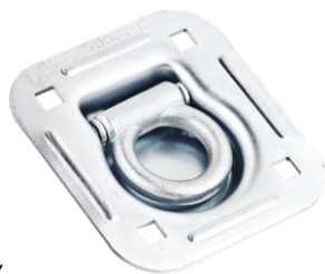
TP1061 Lashing Ring Size:115×124mm, Steel,zinc plated Drain hole in base
